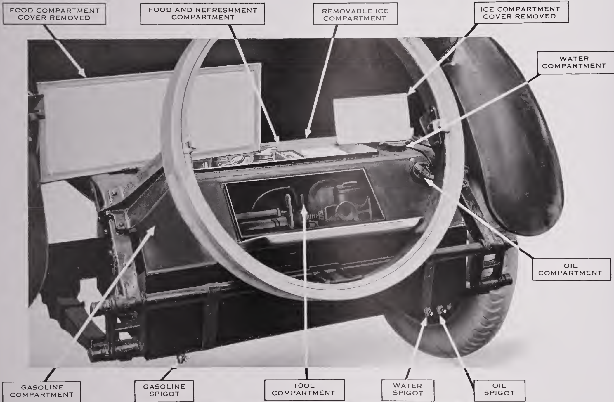
PANDOLFO COMBINATION COMPARTMENT TANK REGULAR EQUIPMENT OF PAN
